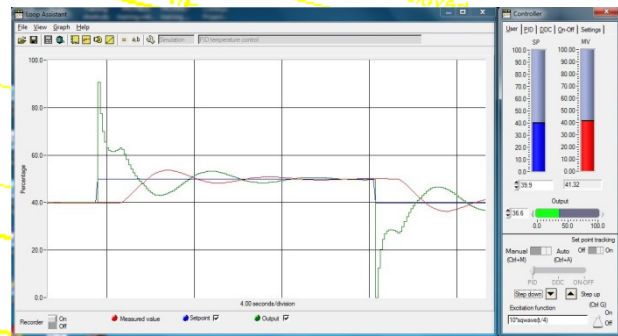
Loop Assistant software used in the training
